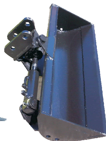
Godet orientable
